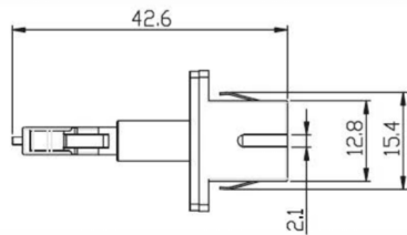
FOA-STF-LCM ST Female to LC Male
