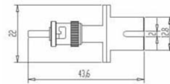
FOA-STF-SCM ST Female to SC Male
